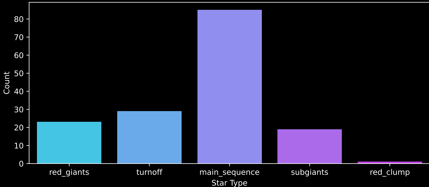
APOGEE DR17 Field: [001-05-O] Count plot of Star Type
