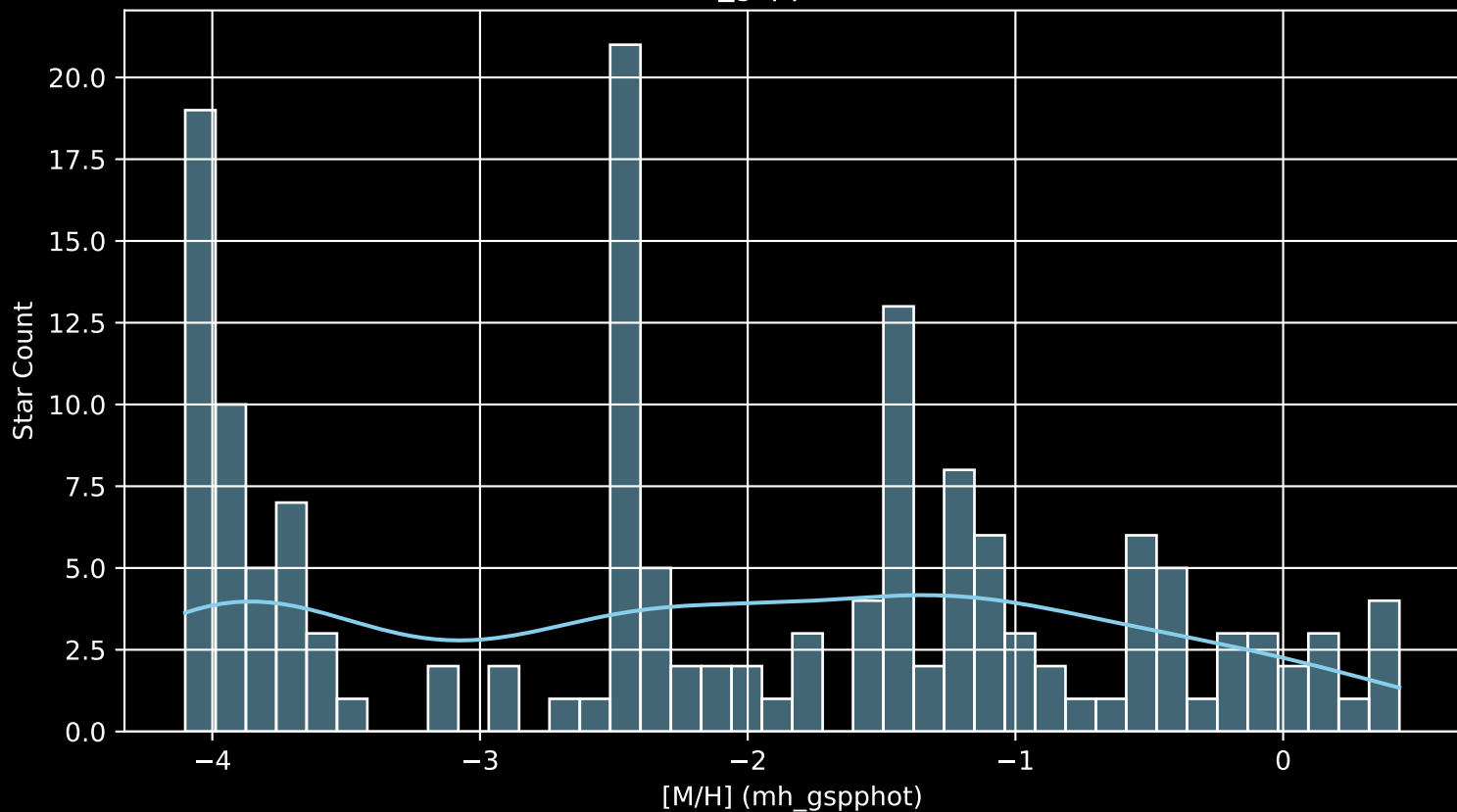
APOGEE DR17 Field: [001-05-O] [M/H] (mh_gspphot) (n= 155)
