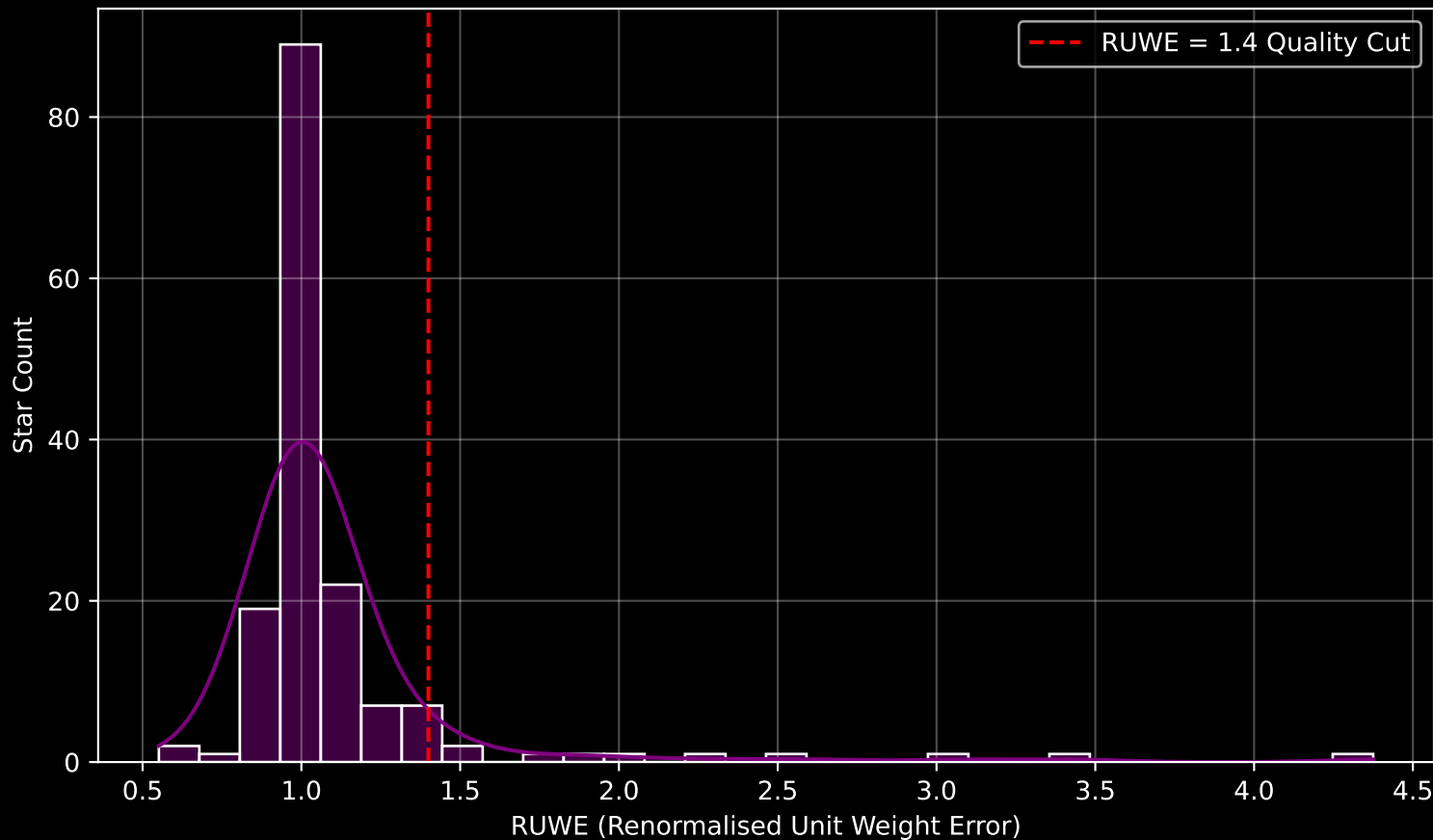
GAPOGEE DR17 Field [001-05-O] RUWE Distribution (n= 157)
