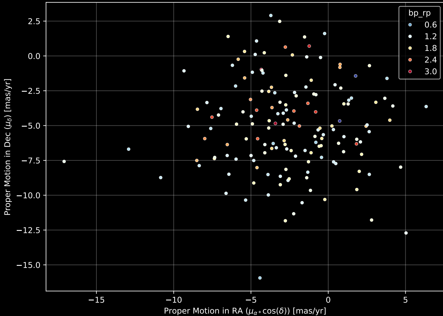
APOGEE DR17 Field: [001-05-O] Proper Motion Diagram (n= 157)
