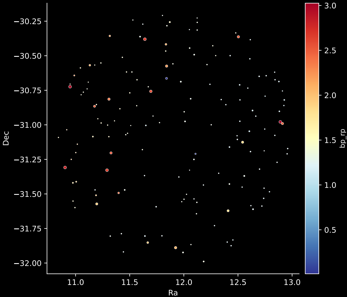
APOGEE DR17 Field: [001-05-O] Stars: 157
