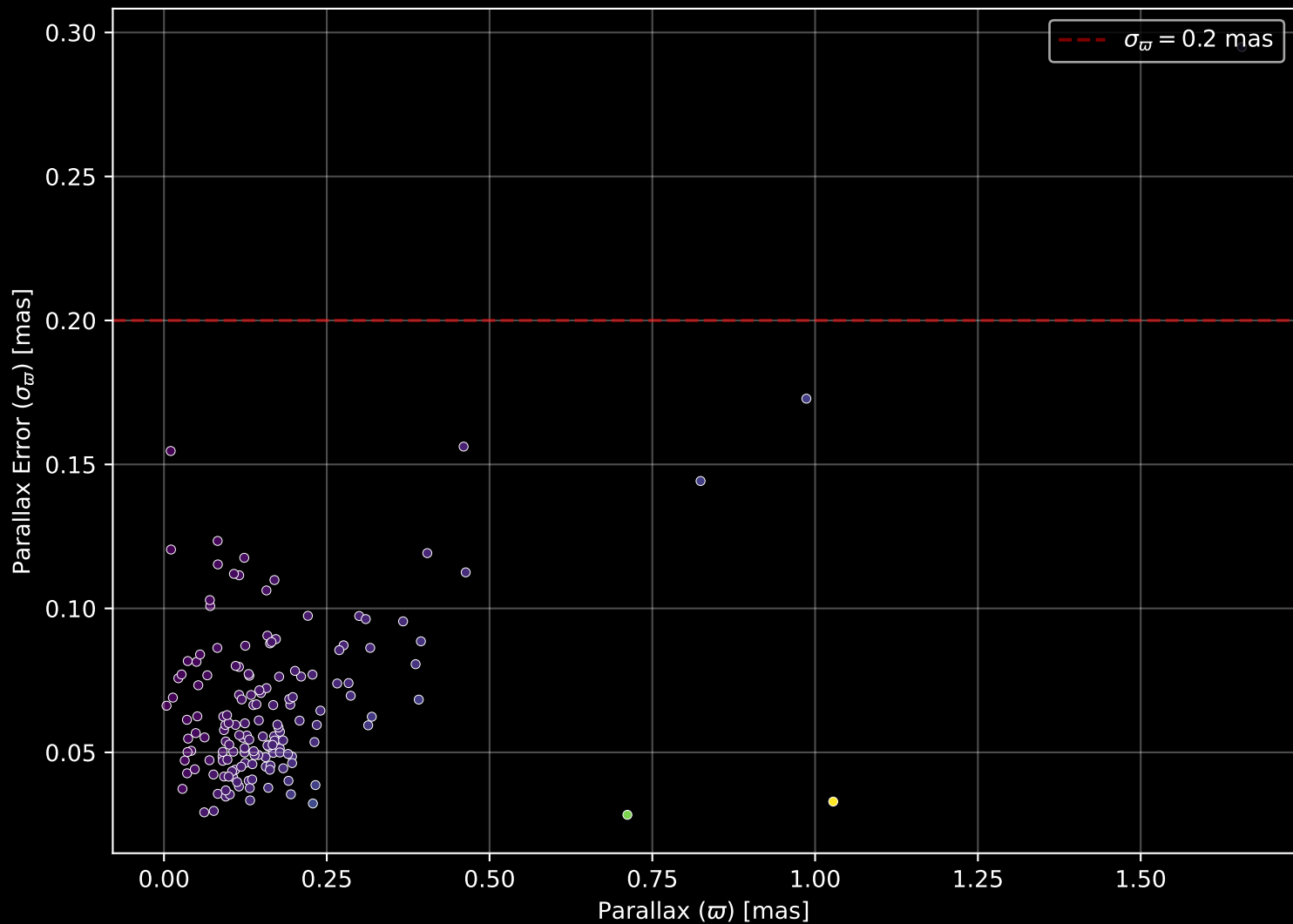
APOGEE DR17 Field: [001-05-O] Parallax Quality (n= 157)
